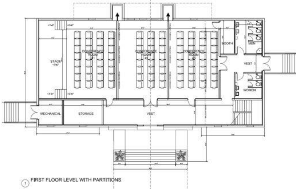
Figure 2, 1 st floor layout without mezzanine illustrated
