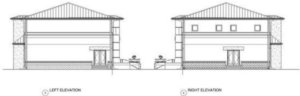
Figure 6, Left and right elevations
