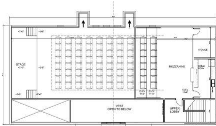
2 MEZZANINE LEVEL
